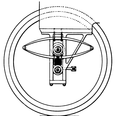
NO. 770,727—PEDESTAL WITH FLANGED ROLLERS.
